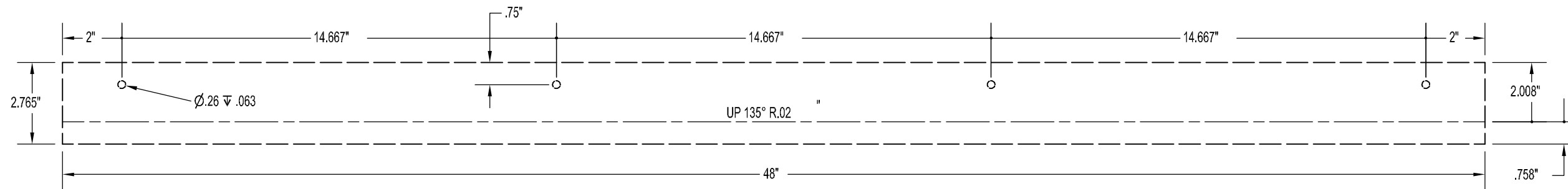
FRENCH CLEAT FLAT PATTERN SCALE 1/4" = 1"
